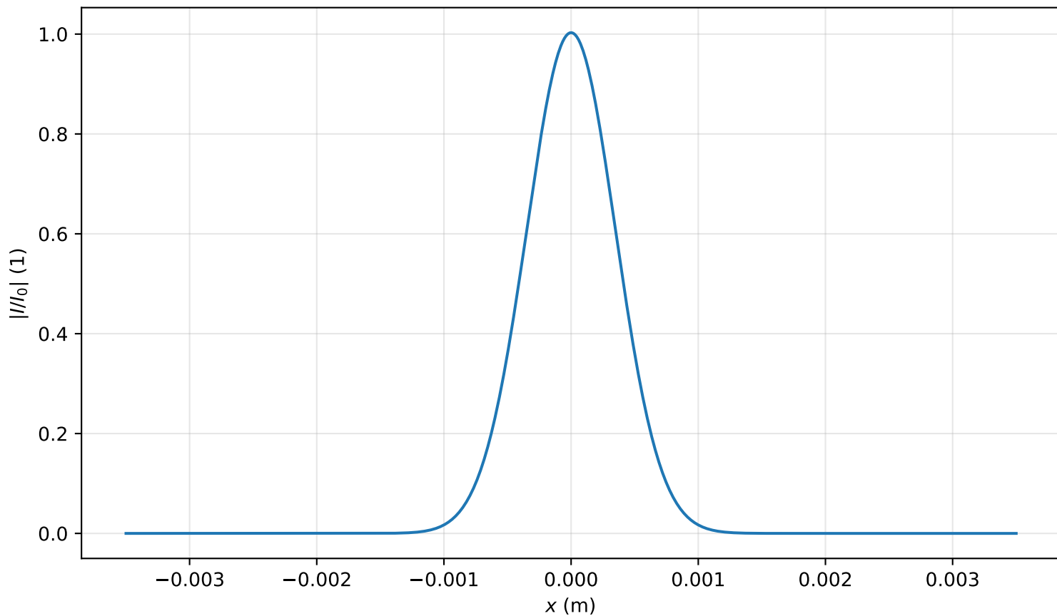
Intensity profile I(x, y = 0, z = 0.080m)/I_0 , P_{in}=0.7P_{cr} , artificial time
